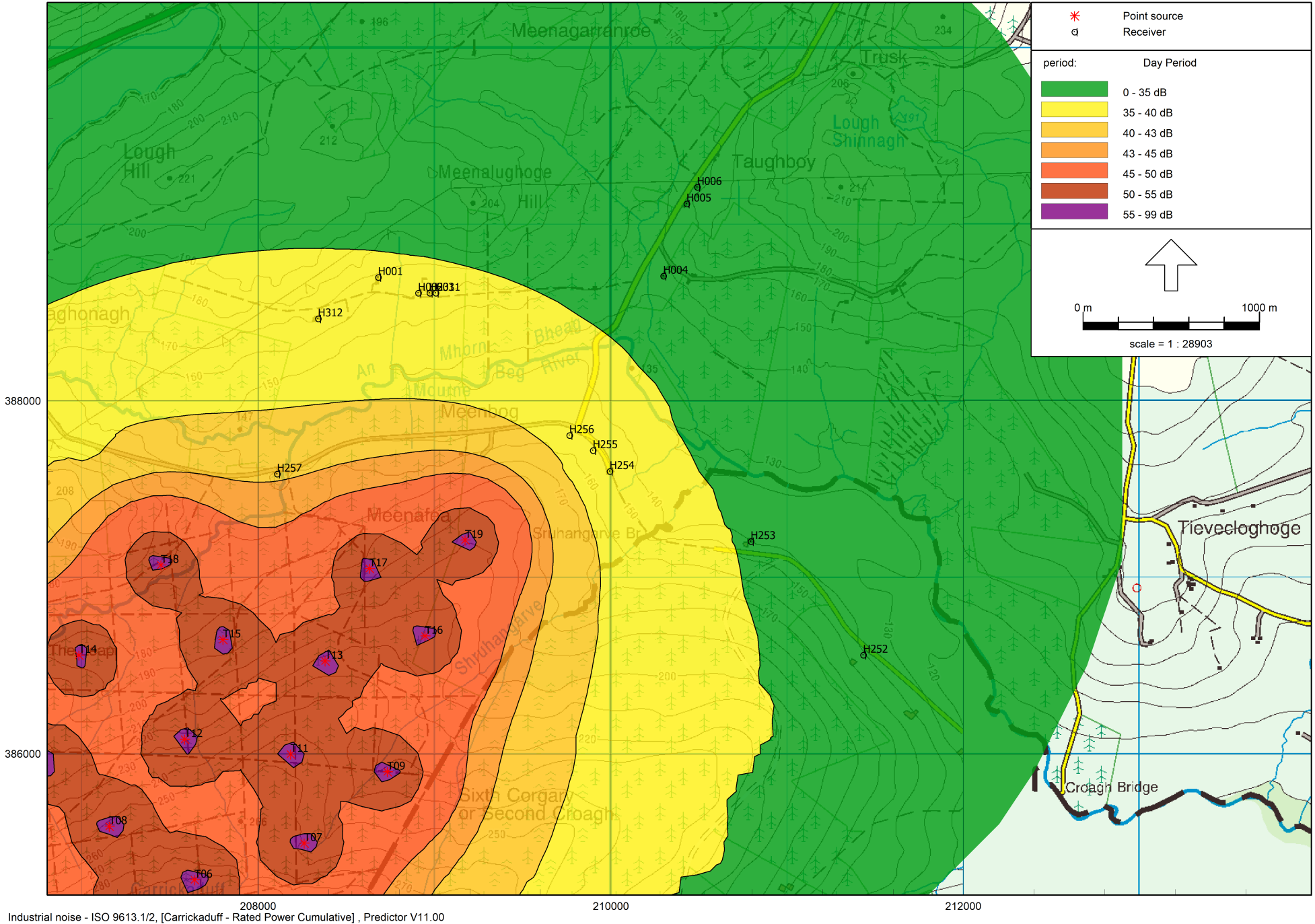
Industrial noise - ISO 9613.1/2, [Carrickaduff - Rated Power Cumulative], Predictor V11.00
